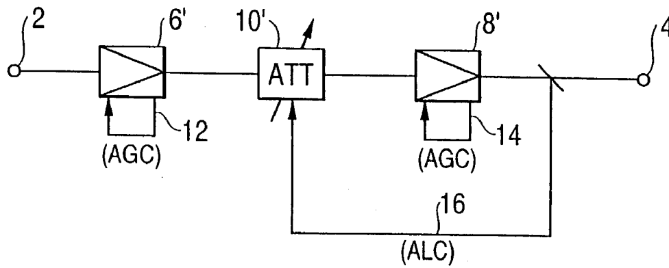
FIG. 3 (PRIOR ART)
